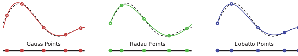
Fig. 19 Illustration showing the three sets of points that are associated with each orthogonal polynomial. In this figure we have shown the Gauss, Radau, and Lobatto points for the fourth-order Legendre orthogonal polynomials. The dashed line in each figure is the same, and the solid lines show the barycentric interpolant that is defined by that set of collocation points. Notice that the interpolant behaves differently for each set of points.
