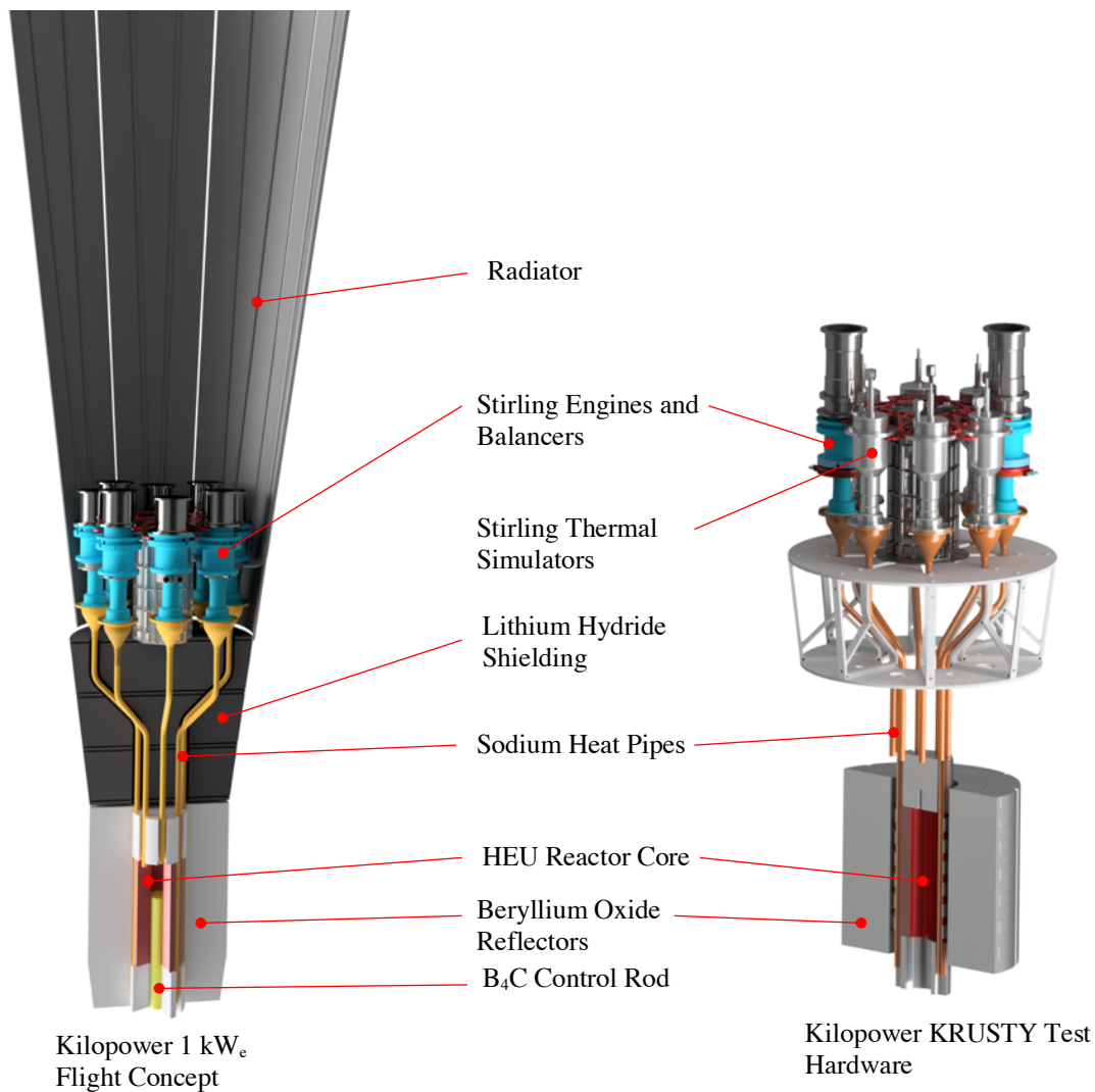
Fig. 1 Kilopower 1 \text{ kW}_e nuclear power system flight concept comparison with KRUSTY nuclear test hardware
